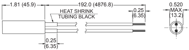
Part Number: CM1000-77C
