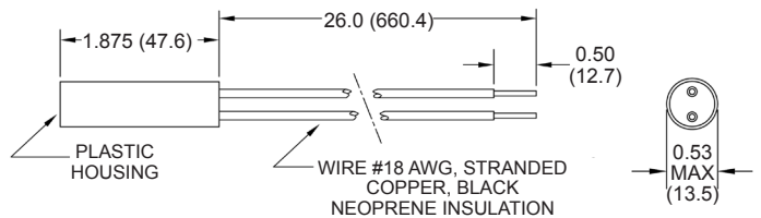
Part Number: CM1000-82
