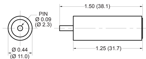
Part Number: CM1000-0
