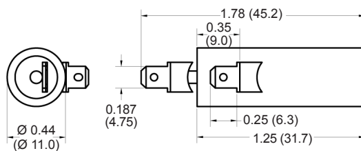
Part Number: CM1000-2
