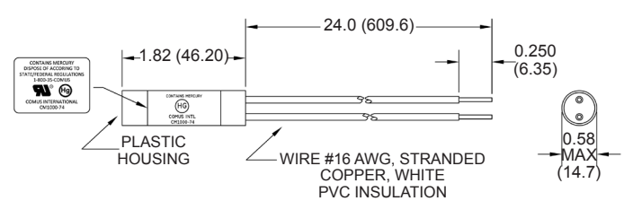
Part Number: CM1000-74
