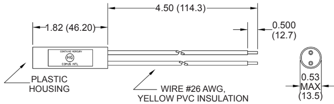
Part Number: CM1000-71
