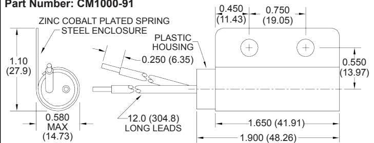
Part Number: CM1000-91
