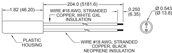
Part Number: CM1000-81
