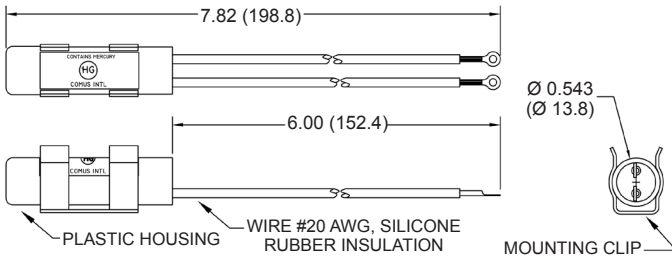
Part Number: CM1000-79
