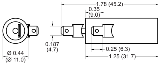
Part Number: CM1000-60
