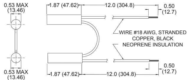
Part Number: CM1000-91
