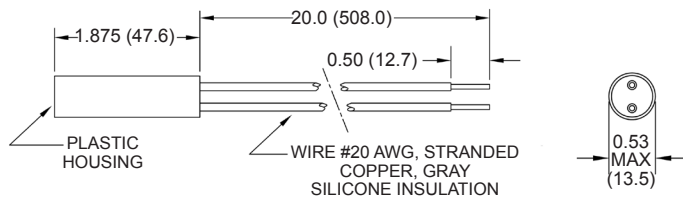
Part Number: CM1000-87
