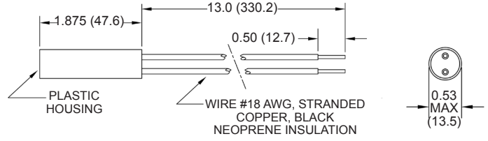
Part Number: CM1000-86
