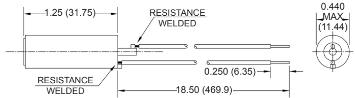
Part Number: CM1000-25
