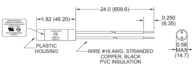
Part Number: CM1000-73
