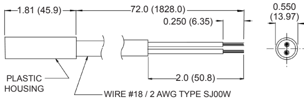
Part Number: CM1000-85
