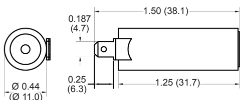
Part Number: CM1000-4
