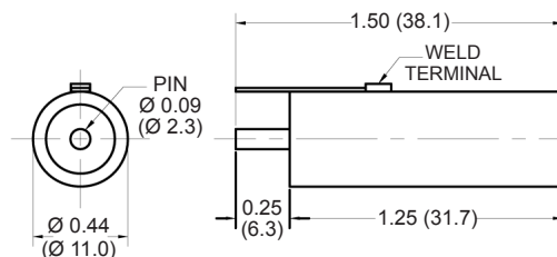
Part Number: CM1000-5
