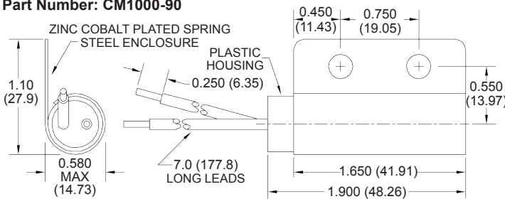
Part Number: CM1000-90
